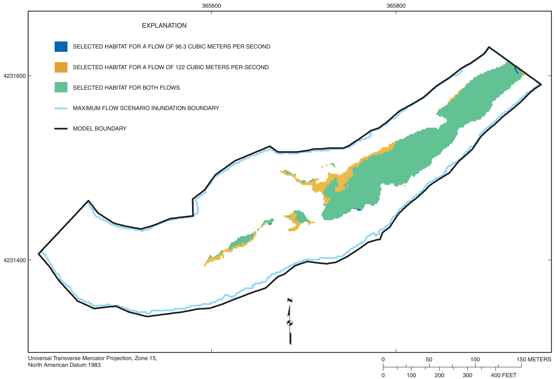
Figure 4-28. Selected habitat area distribution for habitat category 7 (paddlefish) at flows of 96.3 and 122 cubic meters per second at Marais des Cygnes River site MDC2.
